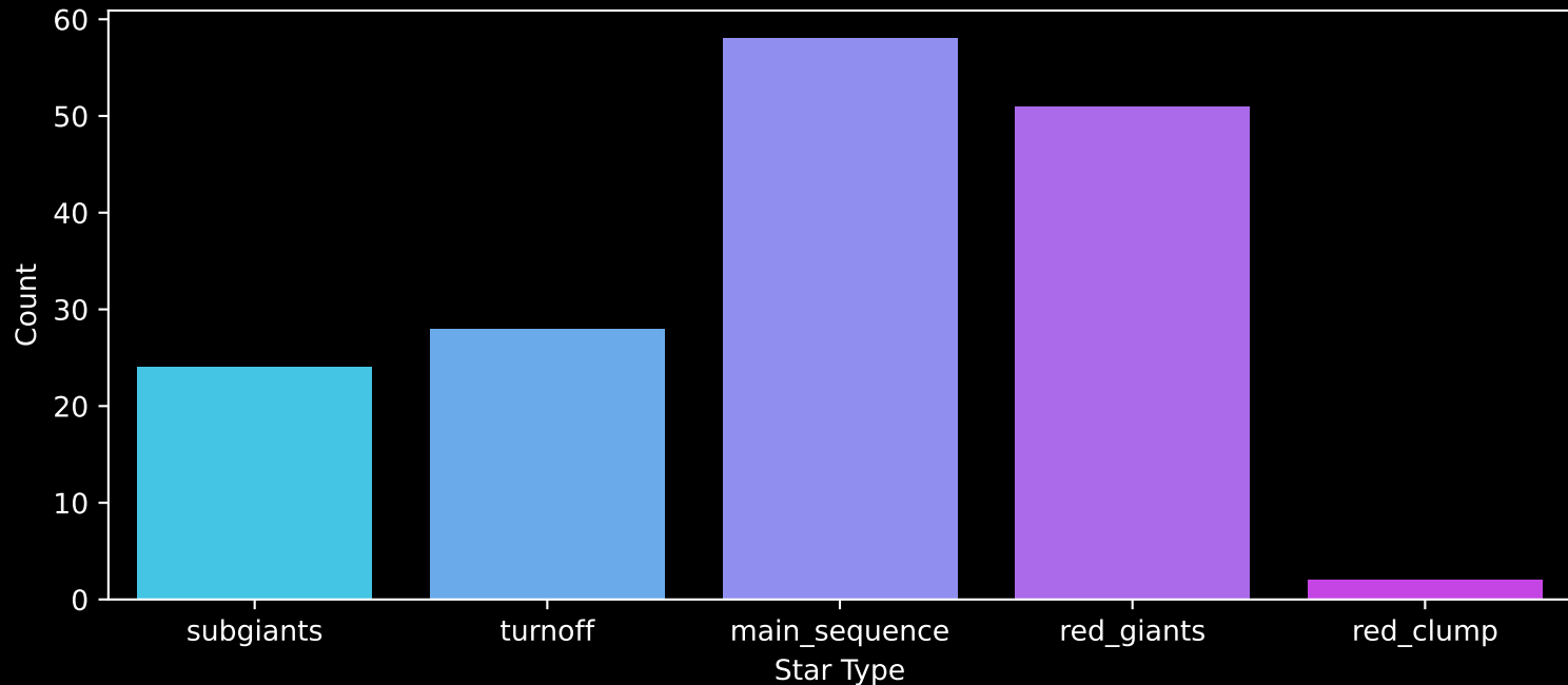
APOGEE DR17 Field: [LMC25] Count plot of Star Type
