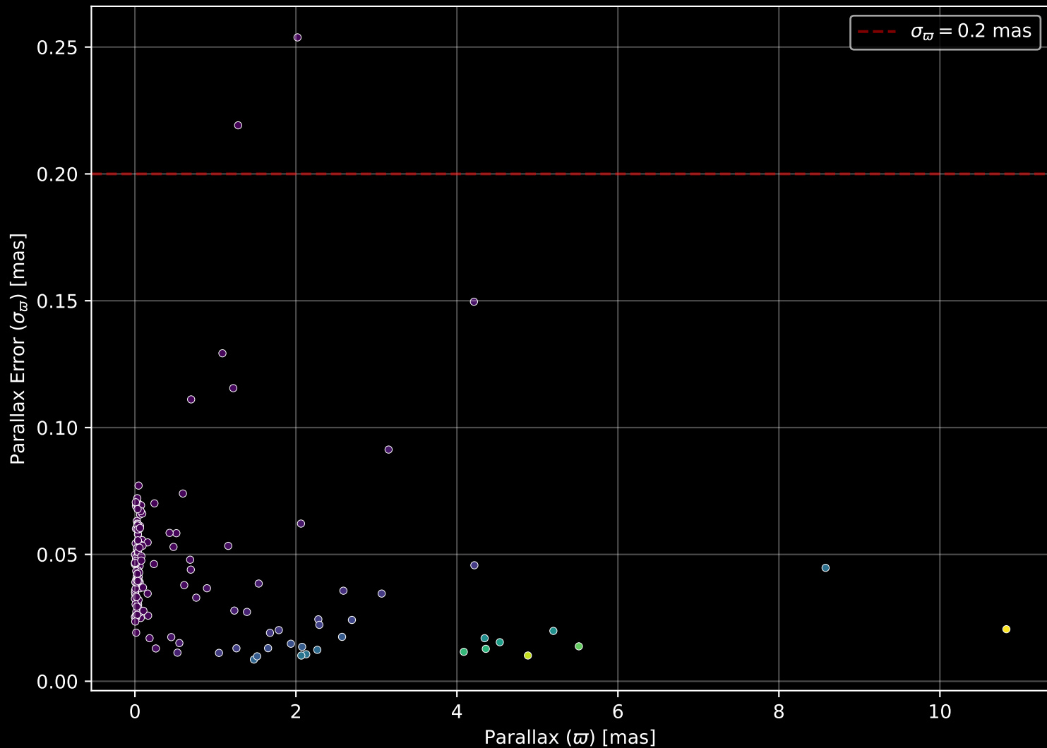
APOGEE DR17 Field: [LMC25] Parallax Quality (n= 163)
