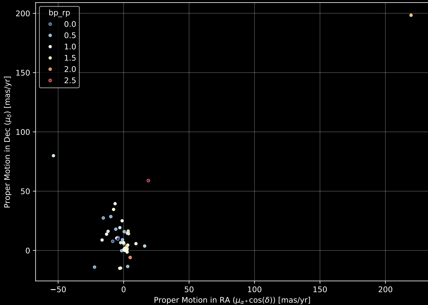
APOGEE DR17 Field: [LMC25] Proper Motion Diagram (n= 163)
