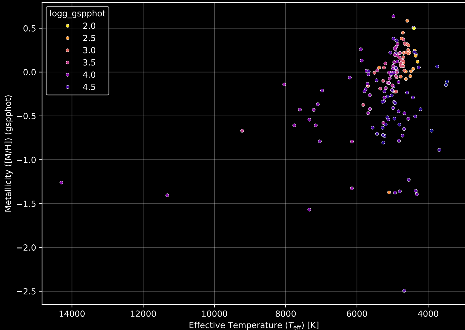
APOGEE DR17 Field: [LMC25] Stellar Population Parameters (n= 163)
