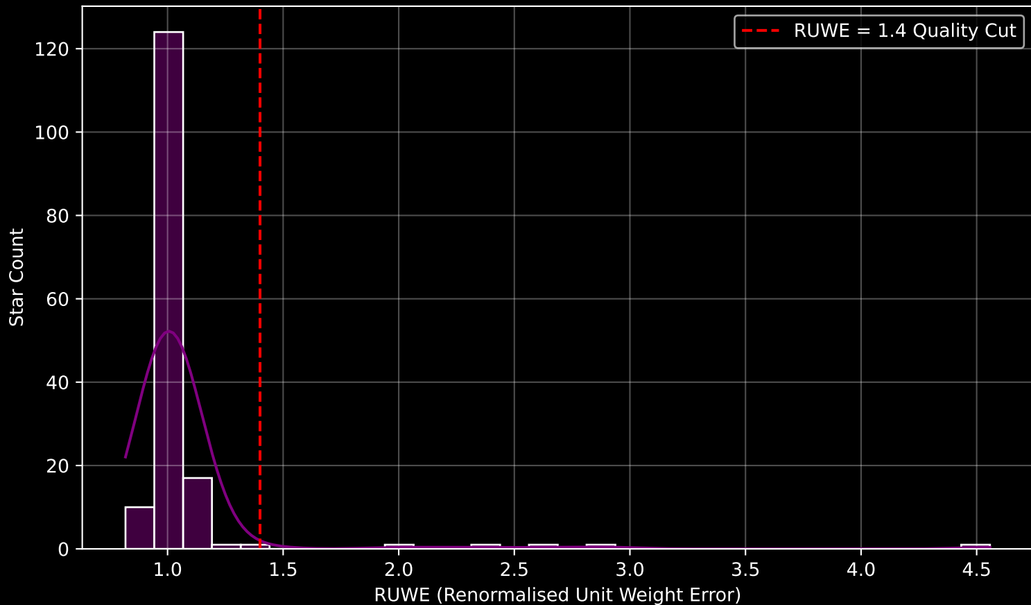
GAPOGEE DR17 Field [LMC25] RUWE Distribution (n= 158)
