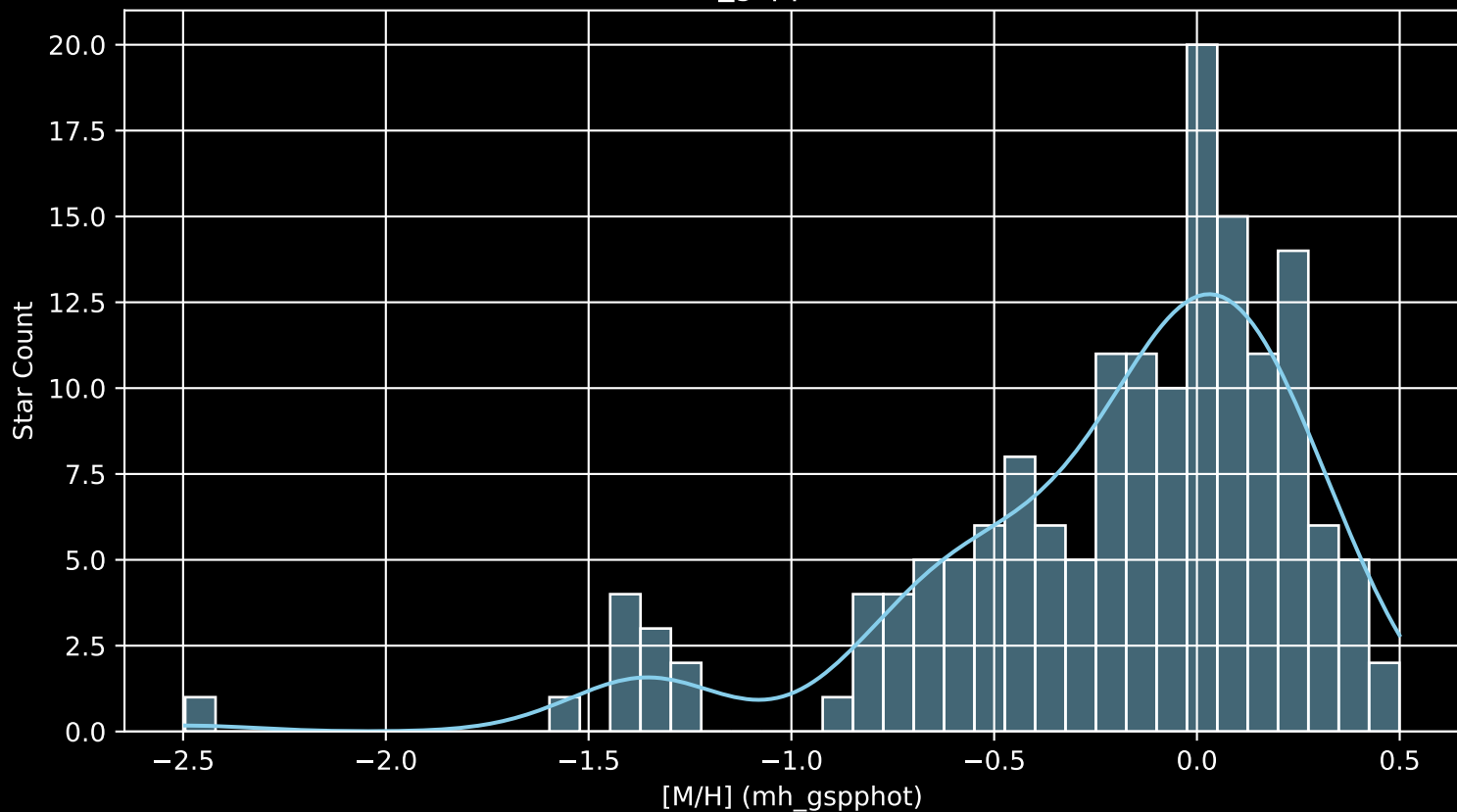
APOGEE DR17 Field: [LMC25 [M/H] (mh_gspphot) (n= 160)
